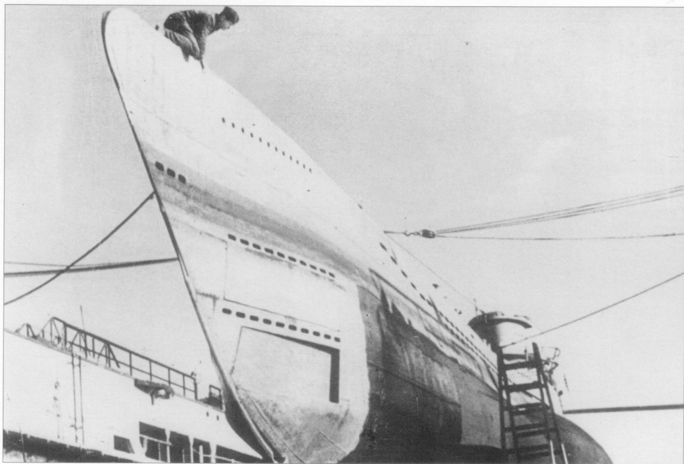
Uboot Typ VII C, w suchym doku, Salamis, 1942. • A Type VII C U-Boat in dry dock, Salamis, 1942.
