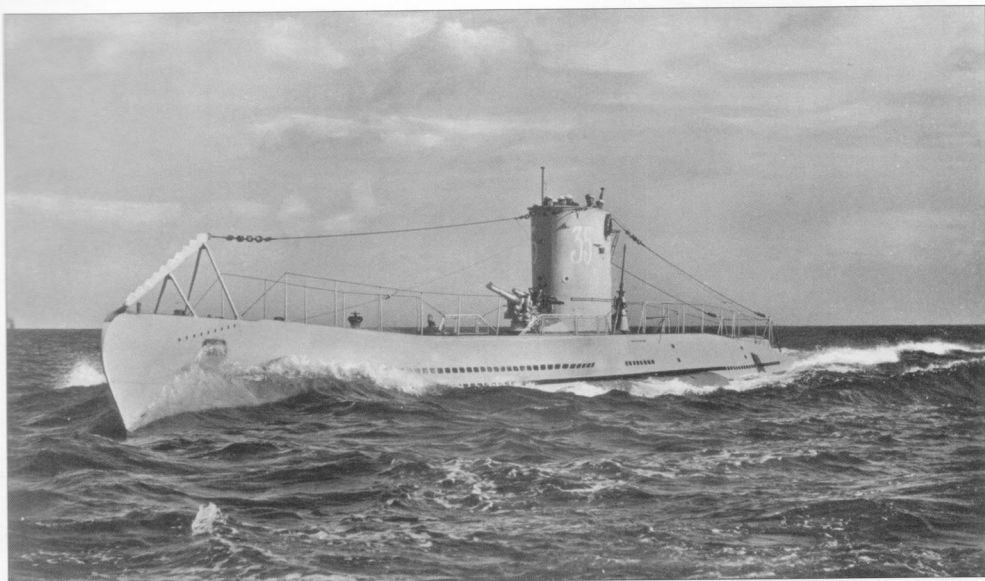
U 35 (Type VII A).
